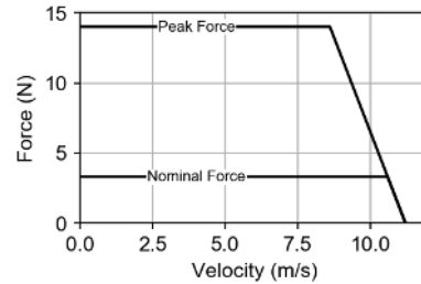
Abb. 11 Force-speed diagram of an iron-core linear motor
